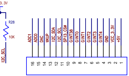
J2 Header 1x16
