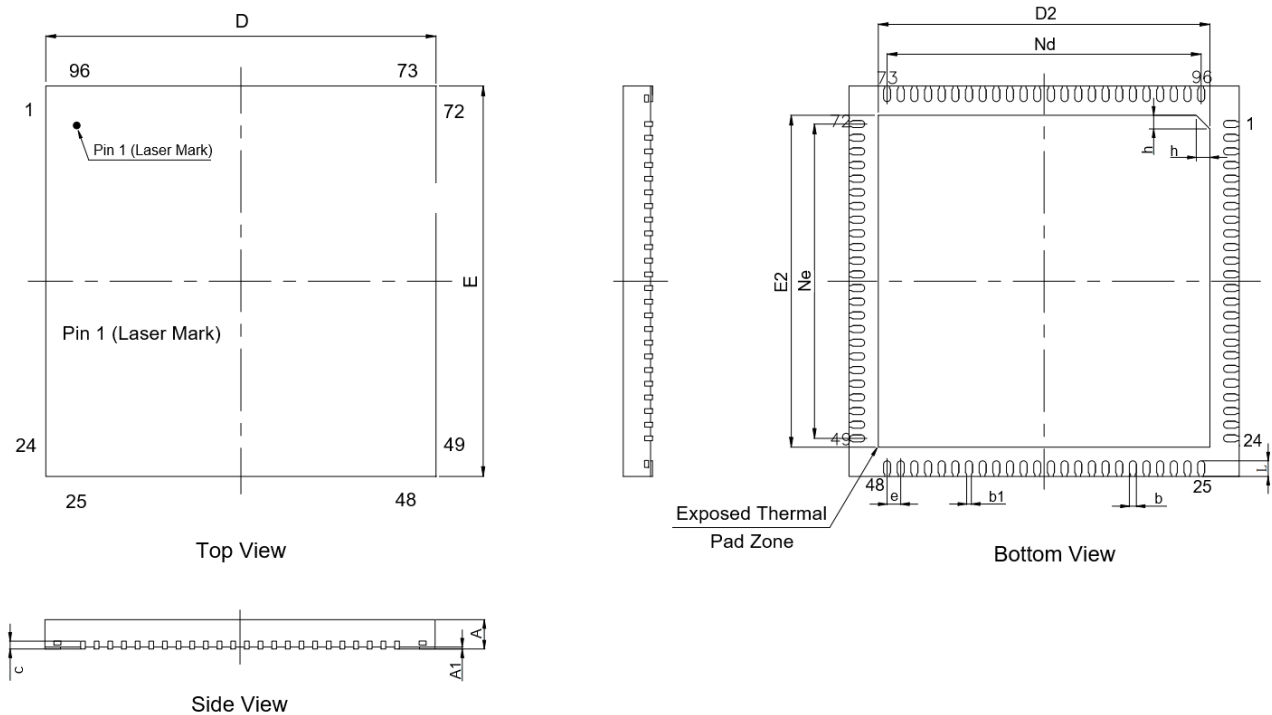
Figure 8-1: QFN-96Pin Outline
